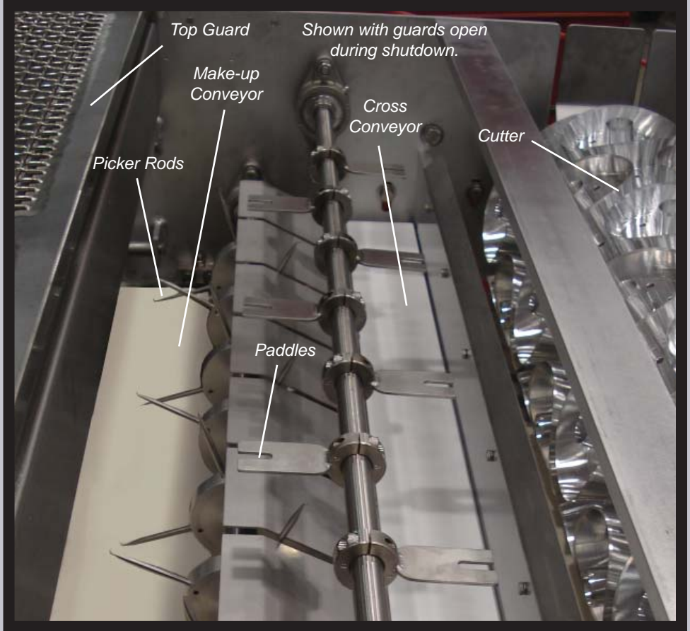
Portable Donut Cutter-Picker Unit (interior)
